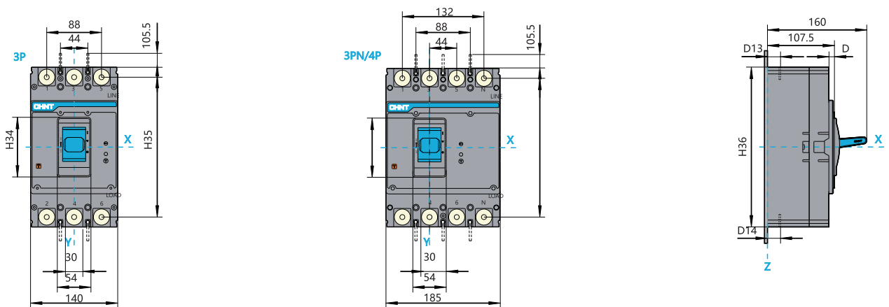
Front connection, dimension (mm)
