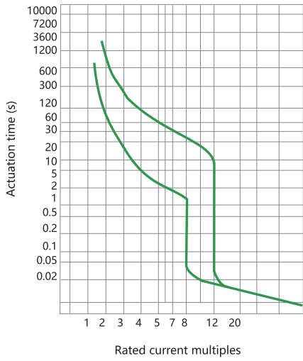
NXM-800
