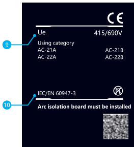
Nameplate of NXHM disconnector switch
