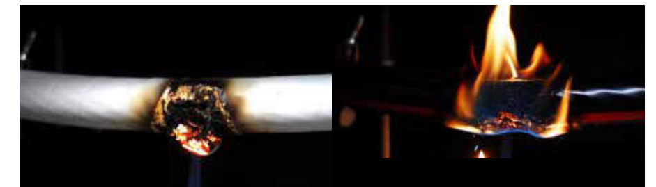
Cable Protected with Scotch® Fire Retardant Electric Arc Proofing Tape 77 During Test
