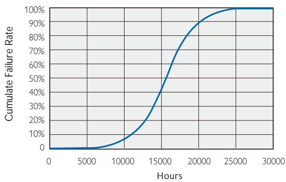
Failure rate vs. Lifetime @ Ta 25 °C
